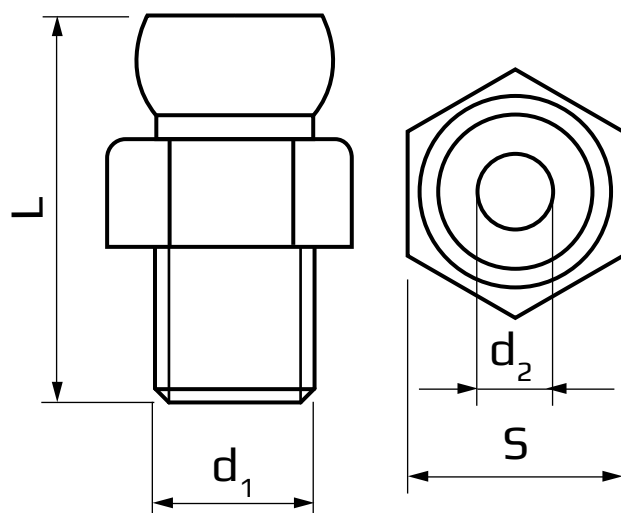
1/2" NPT
